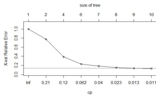
Figure 3. Relative error based on complexity parameter
