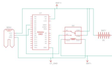
Figure 3: Schematic view
