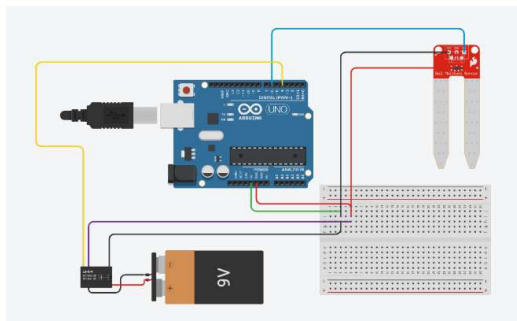
Figure 2: Circuit view
